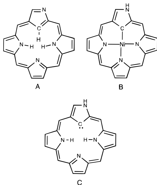
FIGURE 11. Carbaporphyrin structures.
